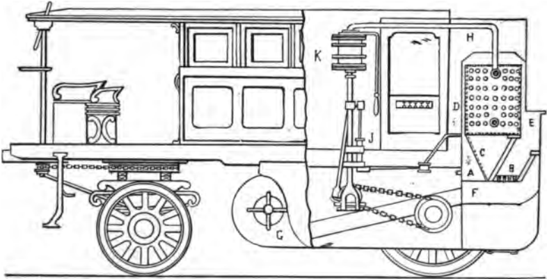
FIG. 6.—Part section of one of Hancock's Coaches, showing Engine and Driving Connections. A is the exhaust pipe leading steam against the screen, C, thence up the flue, D, along with smoke and gases from the grate, B. E is the boiler; H the out-take pipe; K the engine cylinder and, J, the water-feed pump; G is a rotary fan for producing a forced draught, and F the flue leading it to the grate.
